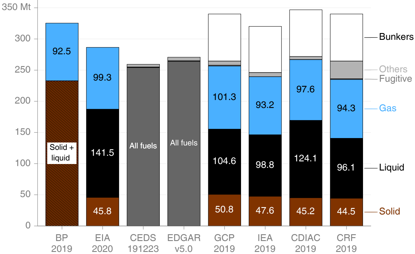
Comparison of fossil CO 2 emissions: BENELUX 2014
