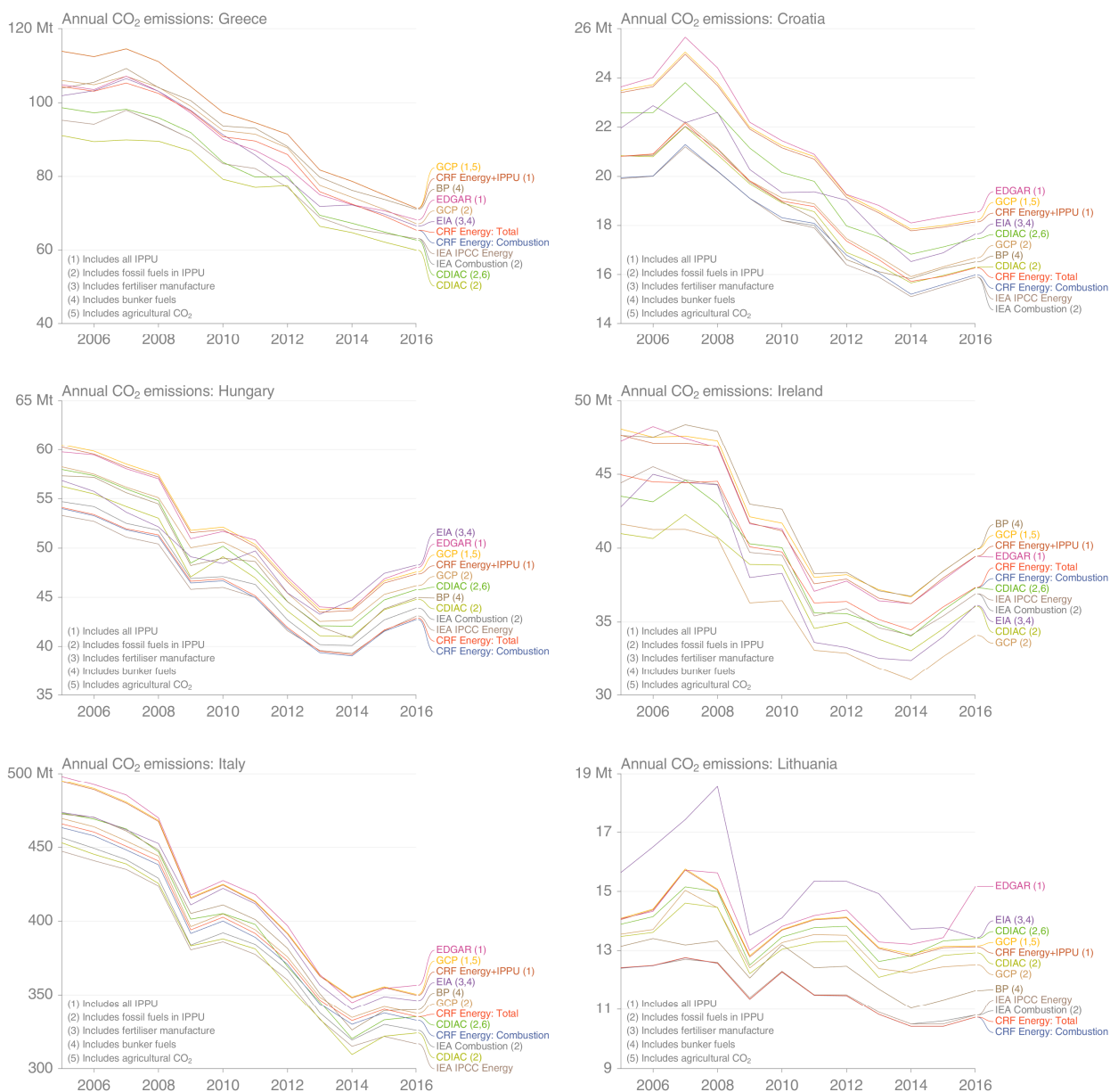
Figure SI-18: Annual CO 2 emissions for EU28 countries from various sources. For details see text.
