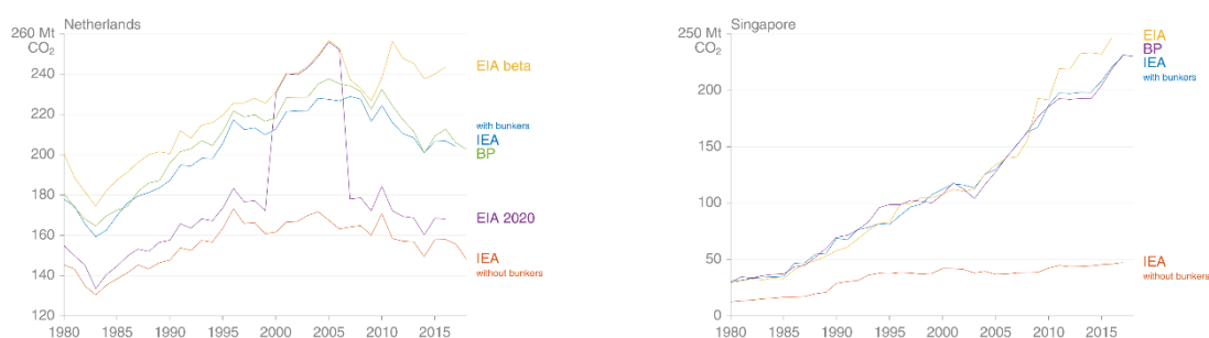
Figure SI-26: The consequences of inclusion/exclusion of bunker fuels varies by country, but is particularly marked for the Netherlands and other, smaller maritime nations (BP, 2019; IEA, 2019a; EIA, 2020, no date). The 2020 edition of the EIA data clearly show an unresolved problem for the Netherlands.
