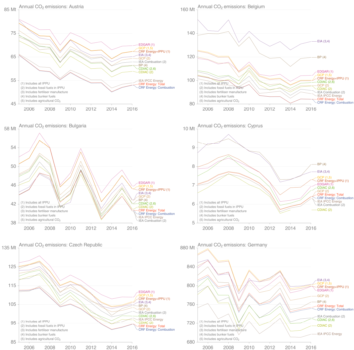
Figure SI-16: Annual CO 2 emissions for EU28 countries from various sources. For details see text.
