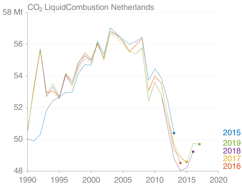
Figure SI-15: Comparison of the five most recent annual Dutch CRF submissions for CO 2 emissions from liquid fuels combustion.
