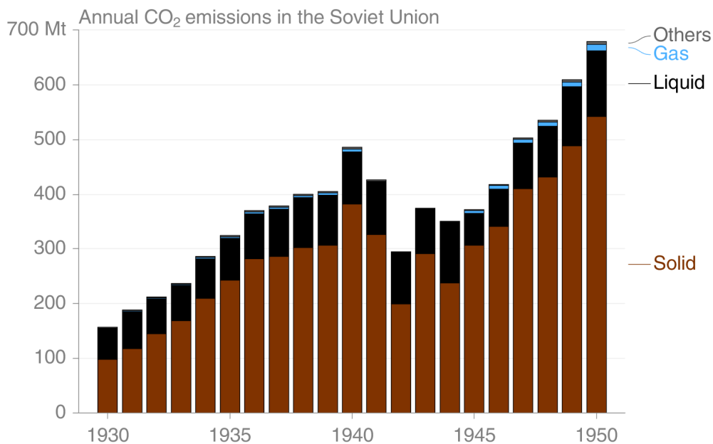
Figure SI-2: Emissions of CO 2 in the Soviet Union, 1930–1950 (Gilfillan et al., 2019).
