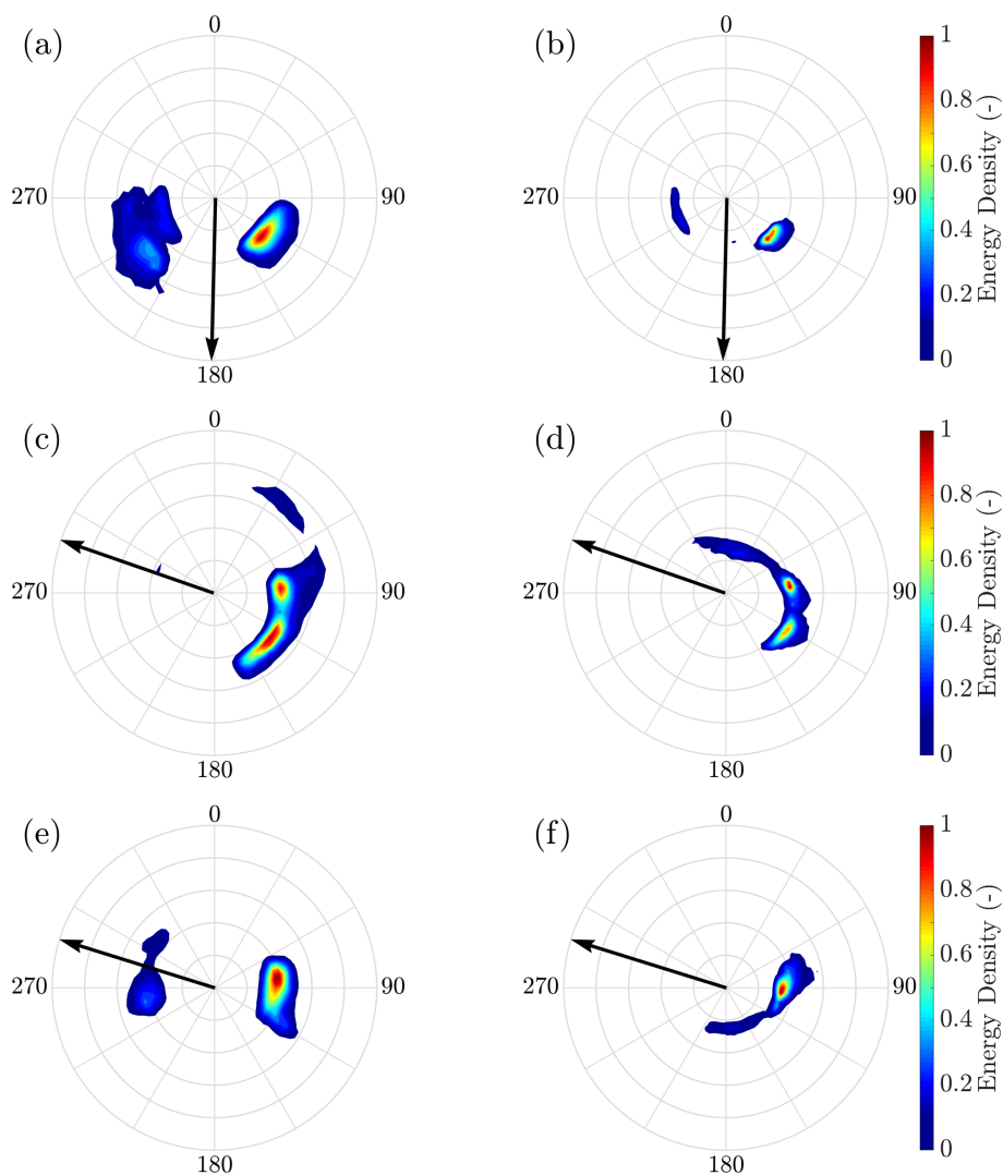
Figure 9. Example directional wave energy spectra recorded during ACE ( a , c , e ) and collocated SAR spectra ( b , d , f ). Wind direction recorded during ACE is shown as black arrows. Both the wave spectra and wind direction follow the “coming from” convention. Circles in the polar plot indicate frequencies from 0.05 Hz (innermost) to 0.25 Hz (outermost) with a step of 0.05 Hz; radiant lines indicate direction with a 30° step.
