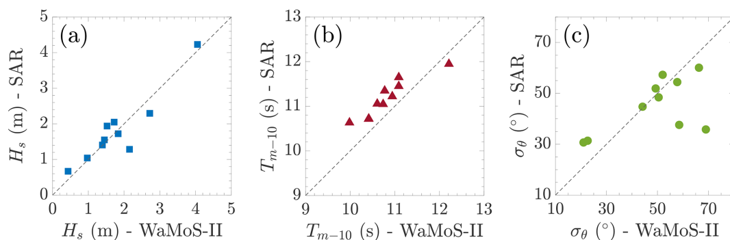
Figure 10. Comparison of integrated parameters (WaMoS-II versus SAR): significant wave height ( H_s , panel a ), energy wave period ( T_{m-10} , panel b ), and wave directional spreading ( \sigma_\theta , panel c ).
