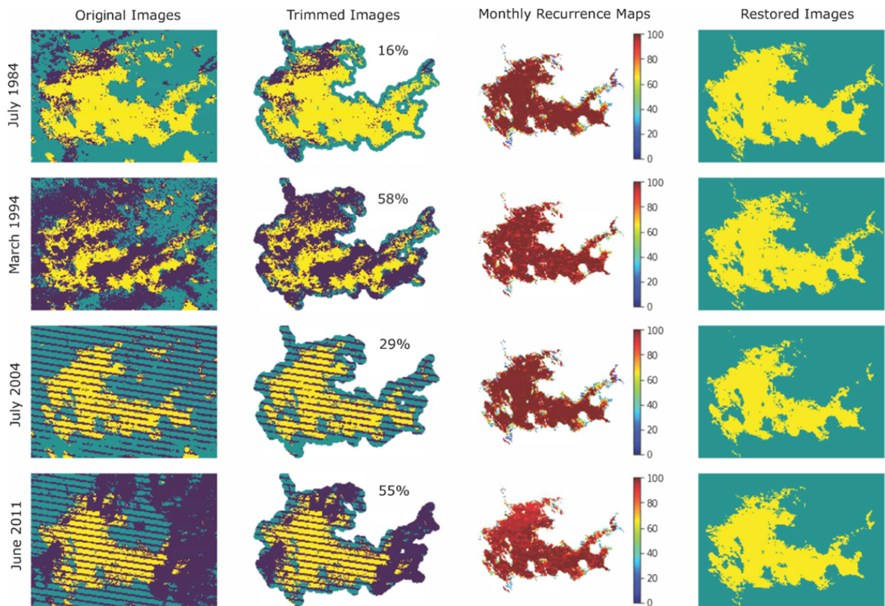
Figure 1. Examples of the performance of the image gap-filling algorithm in Lake Rossignol, Canada. First column, historical water maps from GSWD (yellow – water, green – land and blue – no data; image contaminated ratio from top to bottom: 16 %, 58 %, 29 % and 55 %); second column, historical water maps trimmed by the lake boundary from HydroLAKES with a 500 m buffer (number: contamination ratio); third column, water recurrence (0 %–100 %) maps at the specific month; and fourth column, restored water maps.
