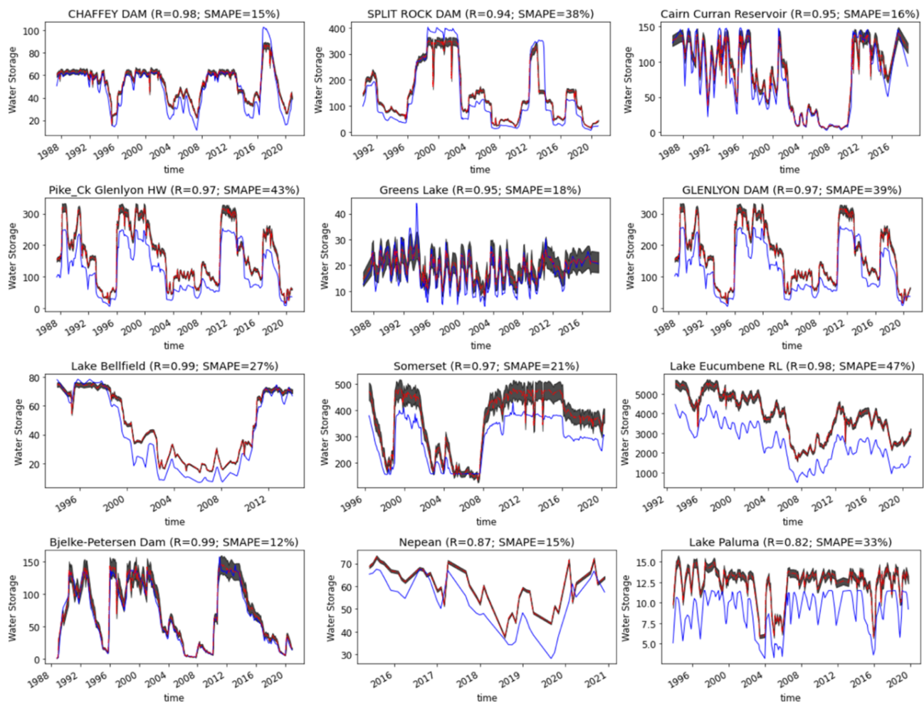
Figure 5. Absolute lake water storage (unit: GL) time series from GloLakes against in situ (observed) data for selected lakes (blue line – observed data, red line – historical storage estimates, black shade – error bars of historical storage estimates).
