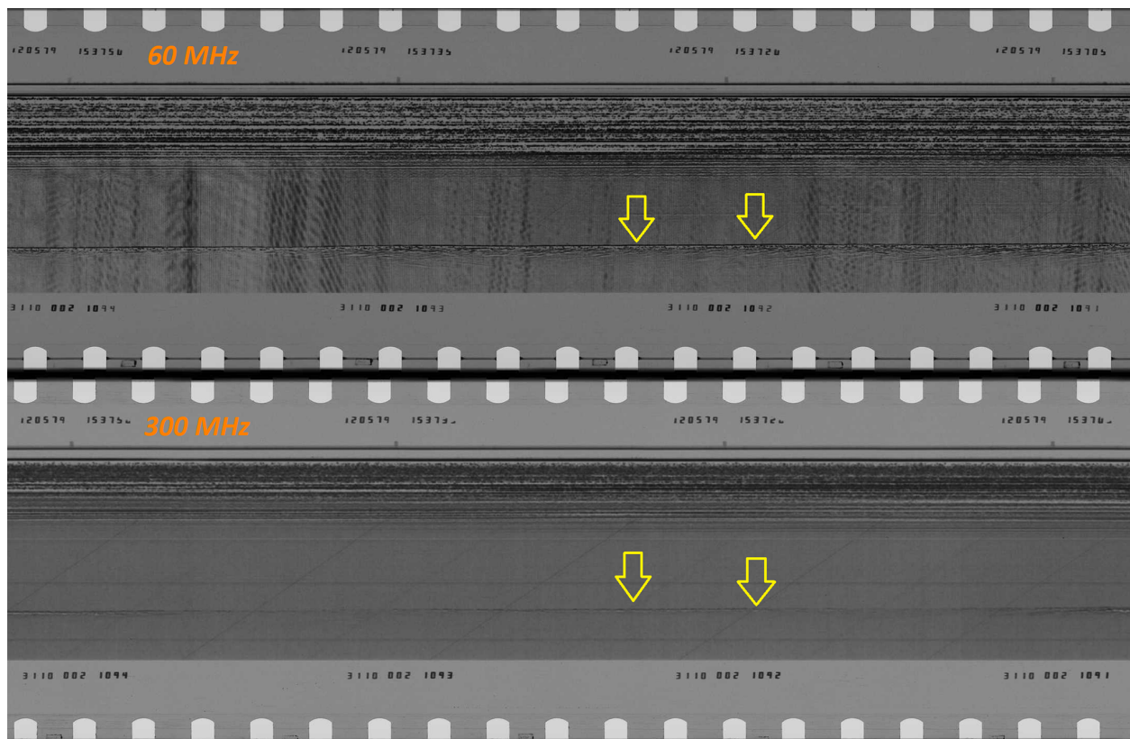
Figure 6. Comparison between 60 and 300 MHz data from flight line 2, 1979. The yellow arrows indicate the bed reflection.
