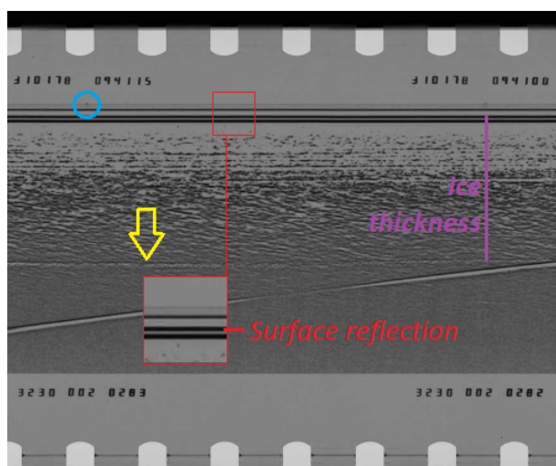
Figure 7. Image file 13_0014525_0014550_lowqual.jpg from flight line 2, 1978, at 60 MHz. The yellow arrow indicates the bed reflection. The insert outlined in red is an enlargement of the surface reflections. The blue circle indicates the exact location of the coordinates tied to CBD 283.
