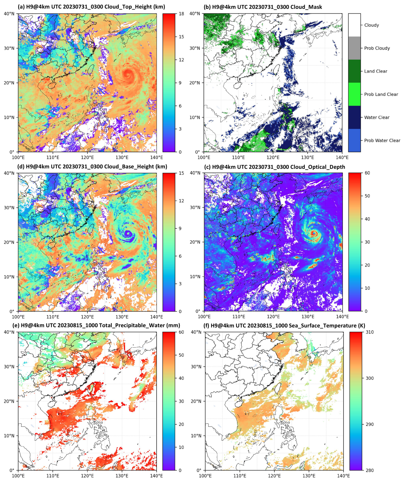
Figure 2. H9/AHI GEO satellite cloud top height (a), cloud mask (b), cloud base height (d), and cloud optical depth (c) at 03:00 UTC on 31 July 2023 and atmospheric total precipitable water (e) and sea surface temperature (f) at 10:00 UTC on 15 August 2023 over the NANO_SCS system.
