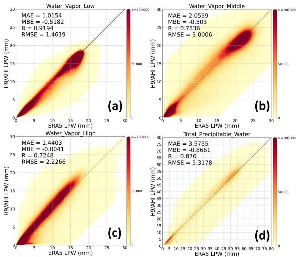
Figure 8. Comparisons of the 1-year (2023) layered precipitable water (LPW) values ( a , low, b , middle, c , high, and d , total) from ERA5 reanalysis and H9/AHI data over the NANO_SCS system. The color bar represents the total number in every bin at an interval of 0.1 mm.
