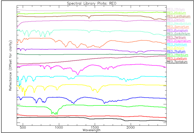
Figure 9: Spectral library plot of the rare earth oxide powders.
