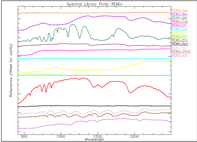
Figure 8: Spectral library plot of the REE-bearing minerals.
