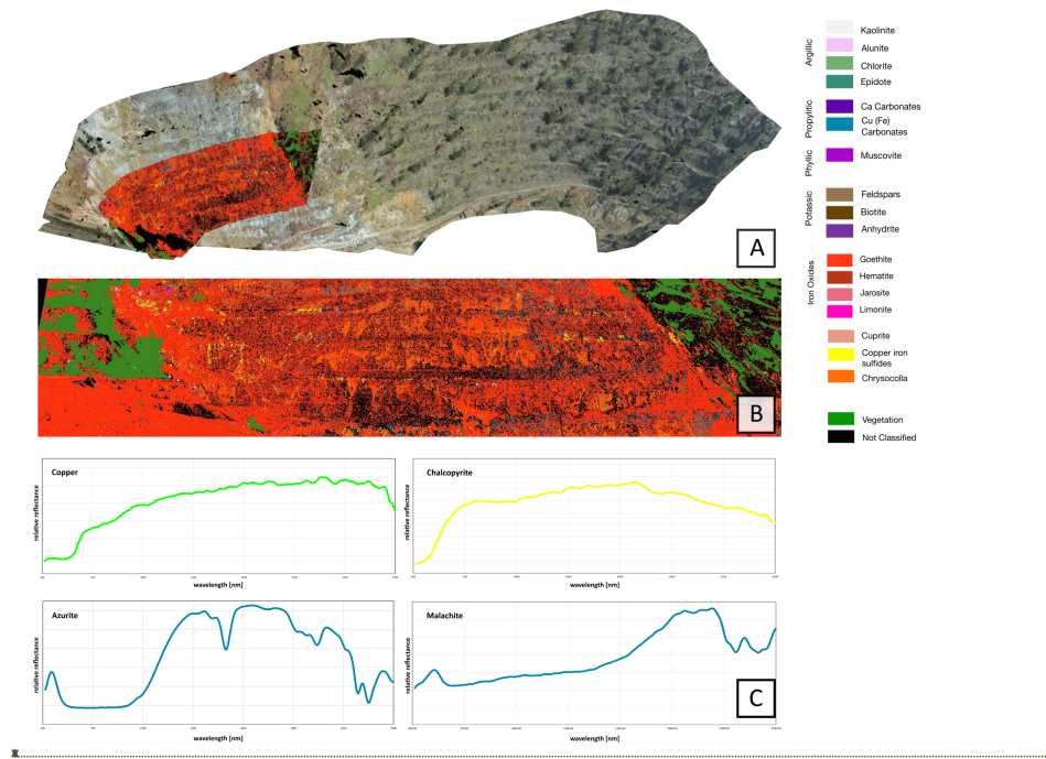
95 Figure 1: Example for the application of a spectral library. A) 3D model of the open pit Apliki mine in the Republic of Cyprus based on RGB images and a superimposed analysis result of a hyperspectral HySpex scan. The hyperspectral map of the spatial mineral distribution from B) is stacked on the 3D model for visualization purposes. B) Analysis of a HySpex scan using a custom-made spectral library from USGS spectra (Clark et al., 2007). C) Example of hyperspectral spectra from copper-bearing minerals as presented in (Koellner et al., 2019).
