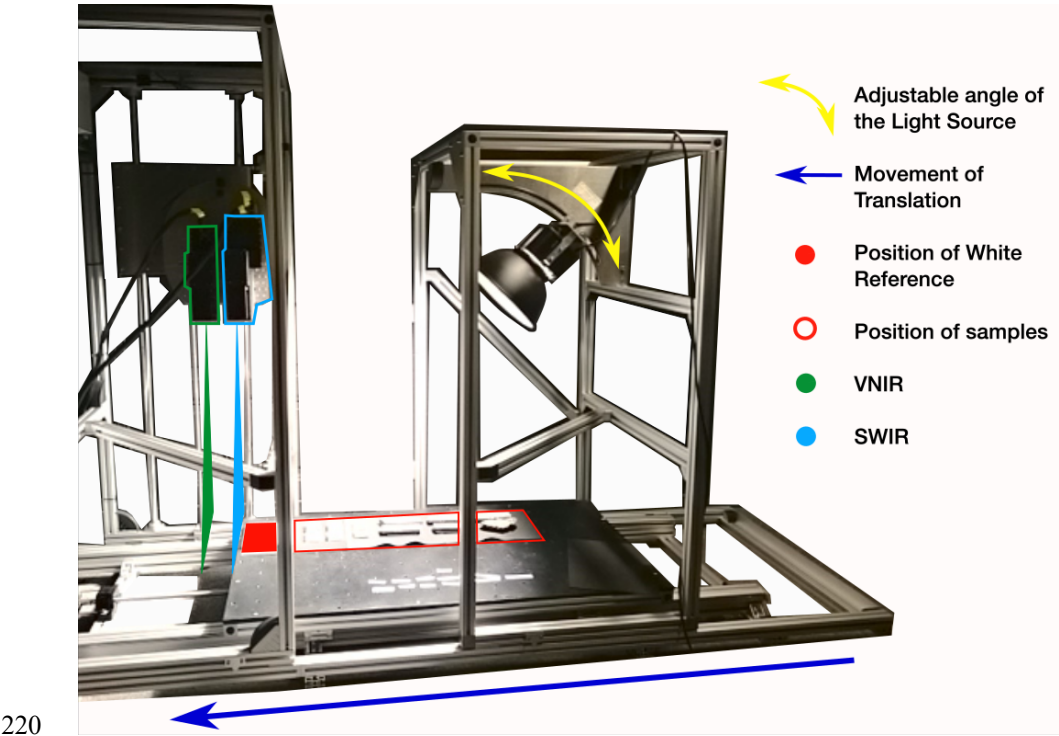
Figure 6: The HySpex translation stage setup (Körting, 2019).
