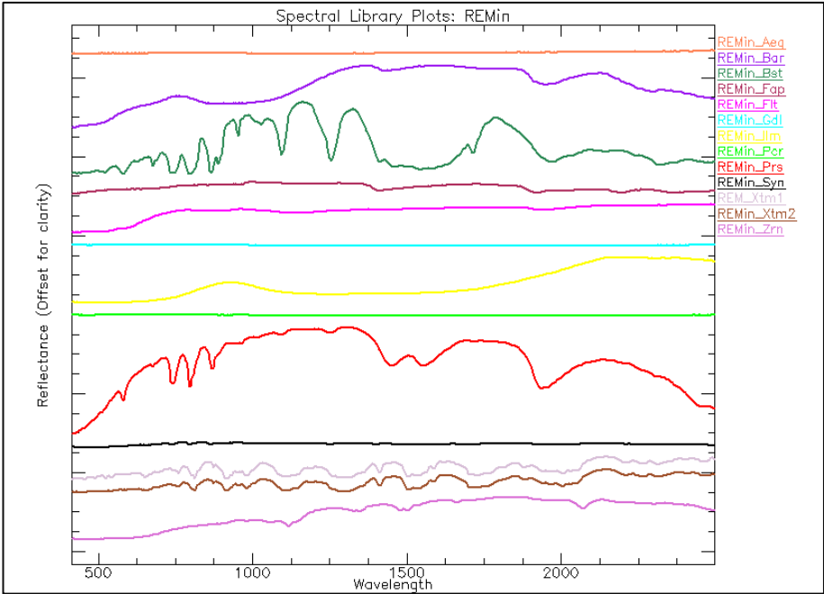
Figure 8: Spectral library plot of the REE -bearing minerals.
