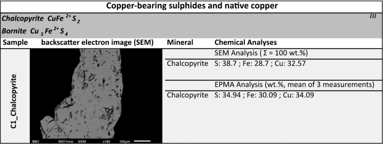
Figure 7: Sample C1_Chalcopyrite SEM and EPMA analysis.
