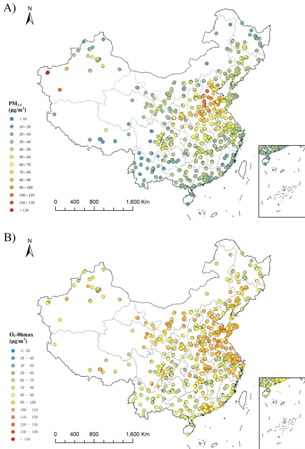
Fig.1 Station distribution in China and average ground monitoring concentration based on the available data of PM 2.5 (A) and O 3 -8hmax (B) from 2013 to 2017
