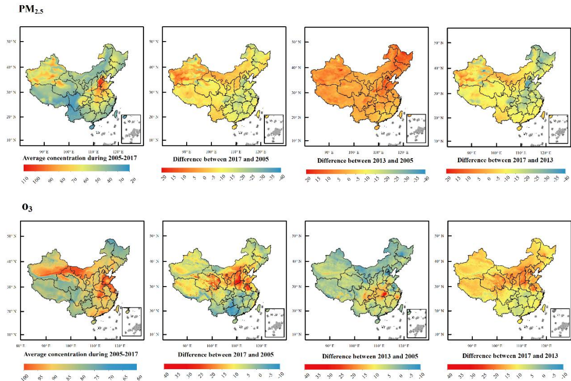
Fig. 6 Estimated annual mean and difference of PM 2.5 and O 3 -8hmax concentration in China during 2005 to 2017
