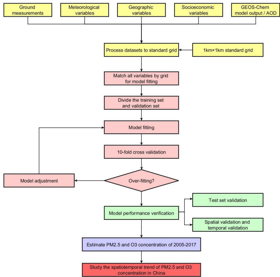
Fig. 2 The workflow of modeling process in the study
