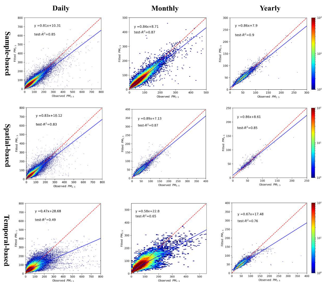
Fig. 3 The density plot of PM 2.5 model
