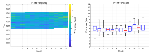
Figure A4. Data screening plot for Torslanda. Left panel shows the data coverage and the monthly mean wind speed value according to the color bar, while the right panel shows the monthly wind speed, where the red line is the monthly mean wind speed, the upper and lower limits of the box 75- and 25-percentile and the end-bars represents the maximum and minimum monthly mean wind speed.
